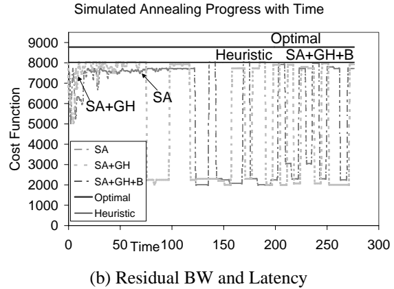
Figure 10. Adaptation performance while mapping 6 VM all-to-all in the challenging scenario.
