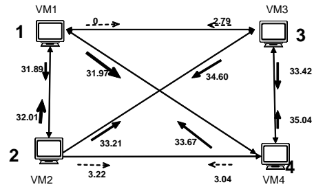
Figure 7. VTTIF topology inferred from NAS MultiGrid Benchmark. Numbers are Mb/sec.
