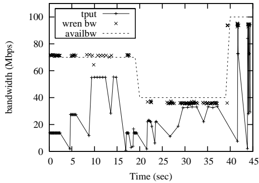
Figure 2. Wren measurements reflect changes in available bandwidth even when the monitored application’s throughput does not consume all of the available bandwidth.
