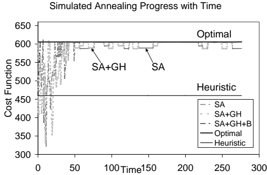
Figure 8. Adaptation performance while mapping 4 VM all-to-all application onto NWU / W&M testbed.
