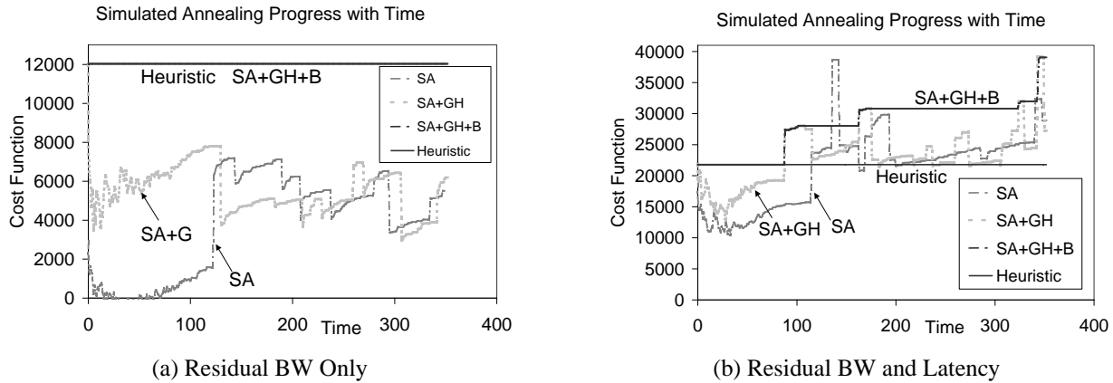
Figure 11. Adaptation performance while mapping 8 VM all-to-all to 32 hosts on a 256 node network.
