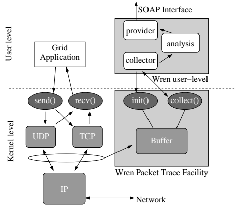
Figure 1. Wren architecture.
