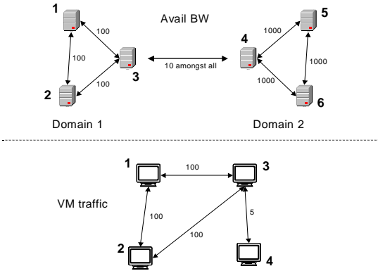
Figure 9. A challenging scenario that requires a specific VM to Host mapping for good performance.
