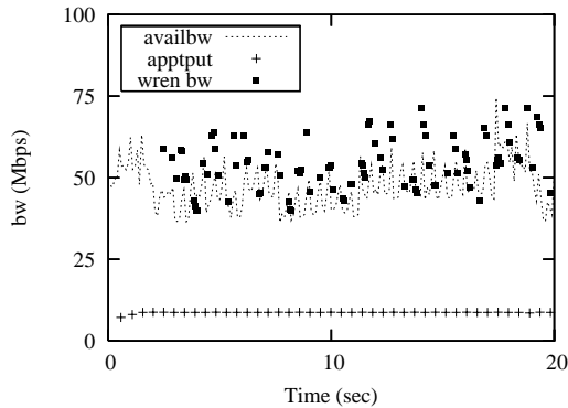
Figure 3. Wren measurements from monitoring application on simulated WAN accurately detect changes in available bandwidth. The cross traffic in the testbed is created by on/off TCP generators.
