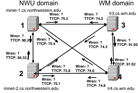
Figure 6. Northwestern / William and Mary testbed. Numbers are Mb/sec.
